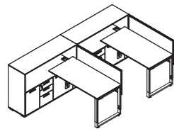
Model:XFS-M1830 Sile:1780Wx3000Dx750/1100H Model:XFS-M1728 Sile:1680Wx2800Dx750/1100H
