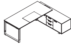
Model:XFS-M2218 Sile:2200Wx1800Dx750H Model:XFS-M2018 Sile:2000Wx1800Dx750H
