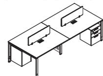
Model:XFS-M2412 Sile:2400Wx1200Dx750H Model:XFS-M2812 Sile:2800Wx1200Dx750H
