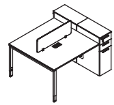
Model:XFS-M1512 Sile:1500Wx1200Dx750/900H
